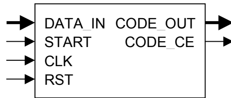
Figure 2. Schematic symbol of the encoder
